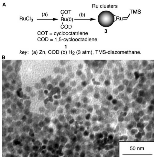
Figure 4. (A) Preparation of ruthenium clusters ( 3 ) with alkylidene linkages. (B) TEM image of ruthenium particles 3 .
