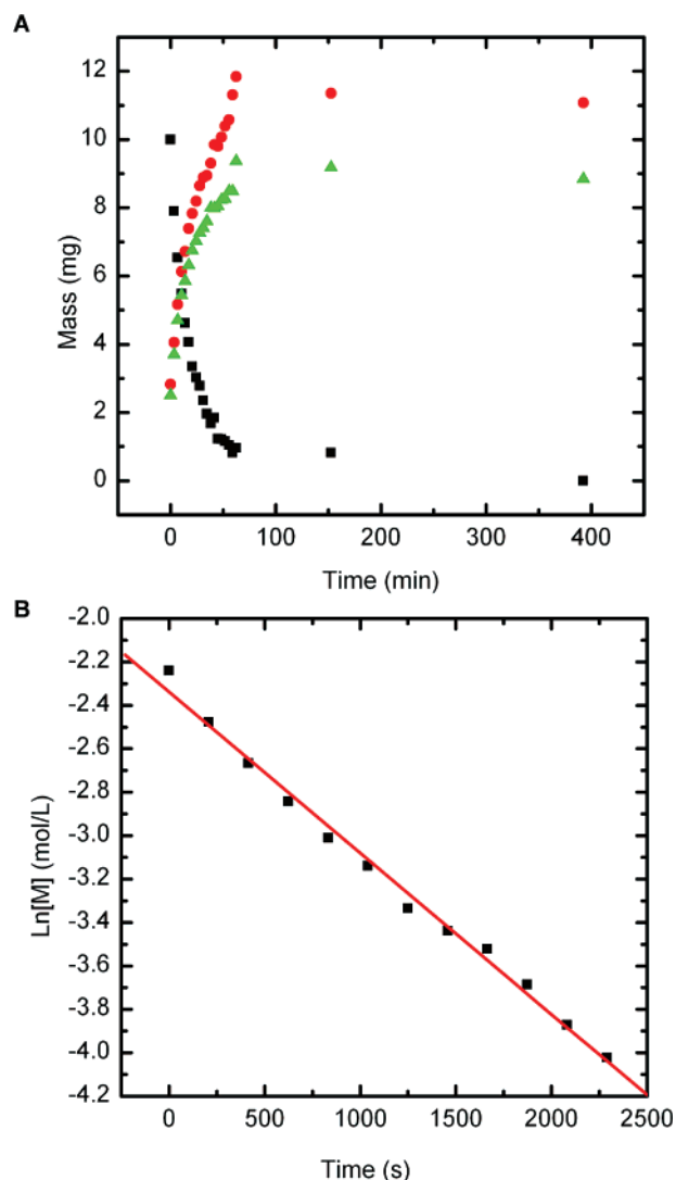
Figure 5. (A) Disappearance of norbornene (black squares) and the appearance of trans (red circles) and cis (green triangles) double bonds in relative to an internal standard (mesitylene) monitored by NMR. (B) Linear fit for the first-order reaction with rate constant k = 7.4 \times 10^{-4} \text{ s}^{-1} , R^2 = 0.993 .
