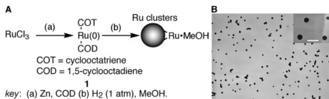
Figure 2. (A) Preparation of ruthenium clusters. (B) TEM image of ruthenium particles. Inset: higher magnification image. The scale bar is 100 nm.
