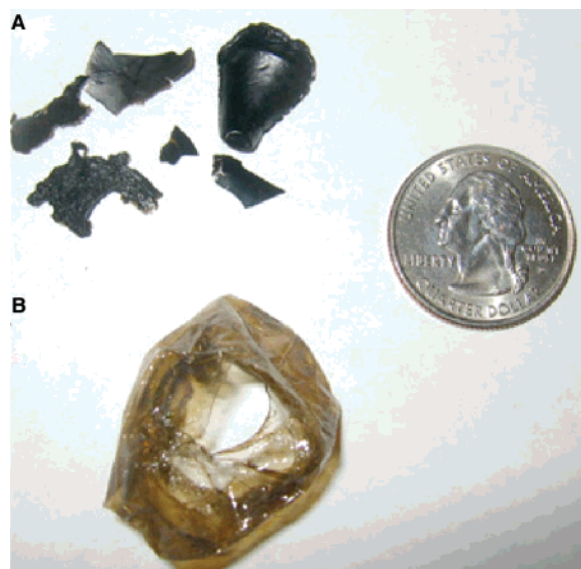
Figure 6. (A) Polynorbornene solid formed by precipitation with methanol then centrifugation. (B) Polynorbornene film made by direct evaporation of the solvent.
