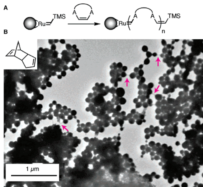
Figure 3. (A) Ring-opening metathesis reaction between a cyclic olefin and surface carbene. (B) Ring-opening metathesis with DCPD. The magenta arrows show areas where polymer is joining particles.
